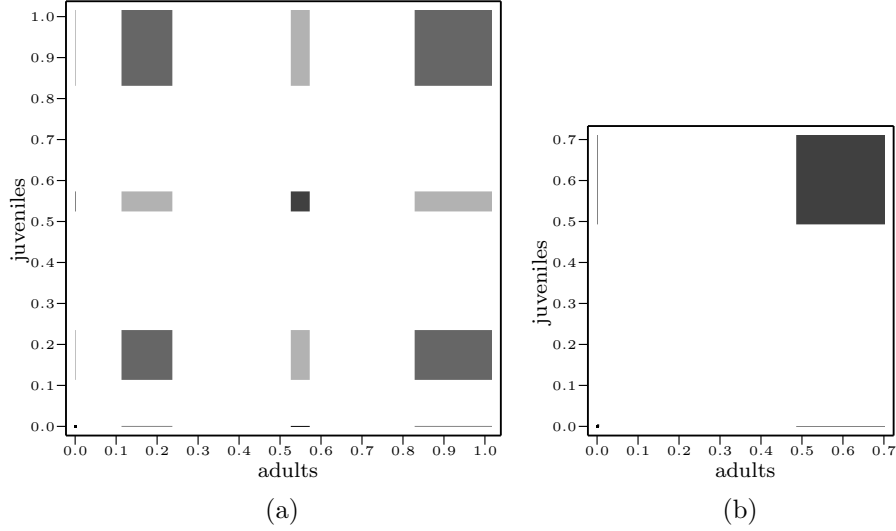
Figure 13: Numerical Morse decompositions that form checkered patterns (resonance) and contain (very thin) isolating neighborhoods along the coordinate axes (synchronization), observed in Case H_a-S_1 for very low values of s_a . The corresponding parameter boxes are: (a) (385, 0): [0.770, 0.772] \times [0.000, 0.002] , (b) (487, 7): [0.974, 0.976] \times [0.014, 0.016] .
