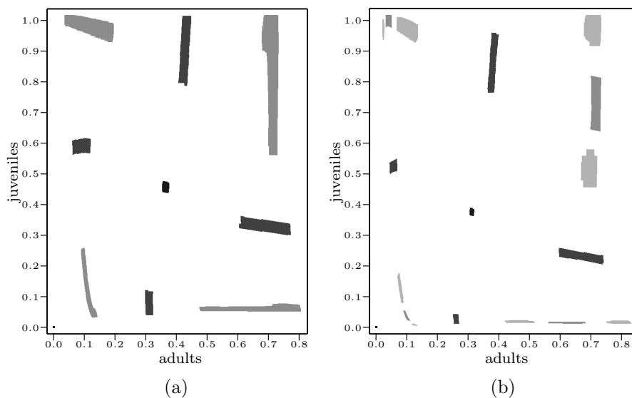
Figure 11: A period doubling bifurcation observed in Case H_a-S_1 . (a) A numerical Morse decomposition observed in Class \mathcal{C}_d . In addition to an unstable neighborhood of the origin (black) and a repelling isolating neighborhood in the center of the picture (grey, blue online), a pair of saddle-type (dark grey, red online) and attracting (light grey, green online) four-periodic isolating neighborhoods are present. (b) In Class \mathcal{C}_{d'} , the attracting four-periodic isolating neighborhood is replaced by a saddle-type four-periodic neighborhood (darker light grey, green online) coupled with an eight-periodic attracting neighborhood (brighter light grey, cyan online). The corresponding parameter boxes are: (a) (307, 144): [0.614, 0.618] \times [0.288, 0.290] , (b) (251, 144): [0.502, 0.504] \times [0.288, 0.290] .
