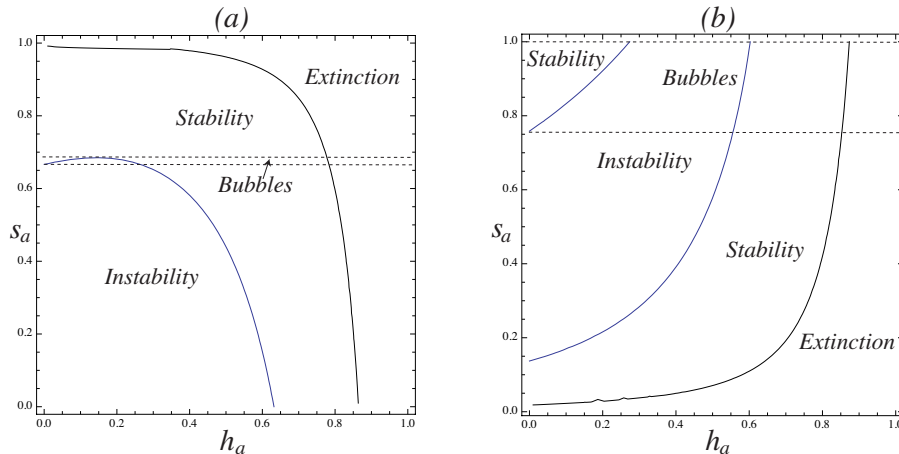
Figure 6: Regions of stability in the plane of parameters (h_a, s_a) for Eq. (6) in Case H_e (equal harvest of adults and juveniles) for r = 4 . (a) Case H_e-S_1 ( s_j = 1 - s_a ). (b) Case H_e-S_e ( s_j = s_a ).
