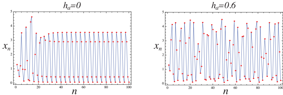
Figure 8: Time series for Eq. (6), Case H_a-S_1 , with r = 4 and s_a = 0.15 . Left: without harvesting (a four-periodic attractor is observed); right: with adult harvest rate h_a = 0.6 (no periodic pattern appears).
