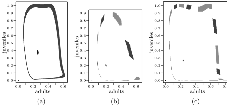
Figure 10: Some saddle-node configurations found in Case H_a-S_1 . (a) An attracting isolating neighborhood in the shape of a ring observed in Class \mathcal{C}_c , with a repeller inside the ring. (b) The ring split into a pair of attracting (dark grey, red online) and saddle-like (bright grey, green online) five-periodic neighborhoods observed in Class \mathcal{C}_{c'} . (c) The ring split into a pair of attracting (dark grey, red online) and saddle-like (bright grey, green online) nine-periodic neighborhoods observed in Class \mathcal{C}_{c''} . The corresponding parameter boxes are: (a) (200, 263): [0.400, 0.402] \times [0.526, 0.528] , (b) (3, 223): [0.006, 0.008] \times [0.446, 0.448] , (c) (118, 185): [0.236, 0.238] \times [0.370, 0.372] .
